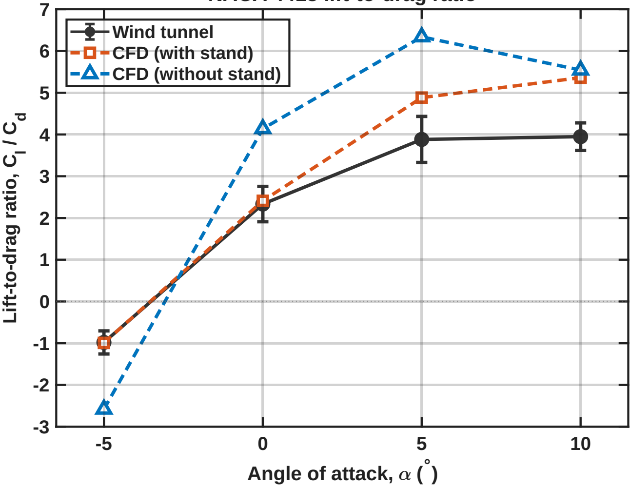
NACA 4418 lift-to-drag ratio
